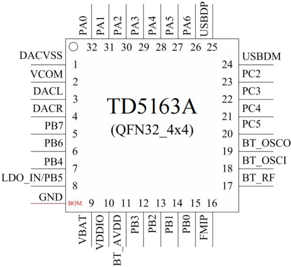
Figure 1-1 TD5163A_QFN32 Package Diagram
